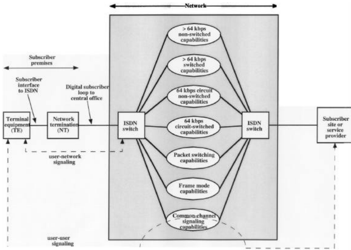
ISDN architecture
