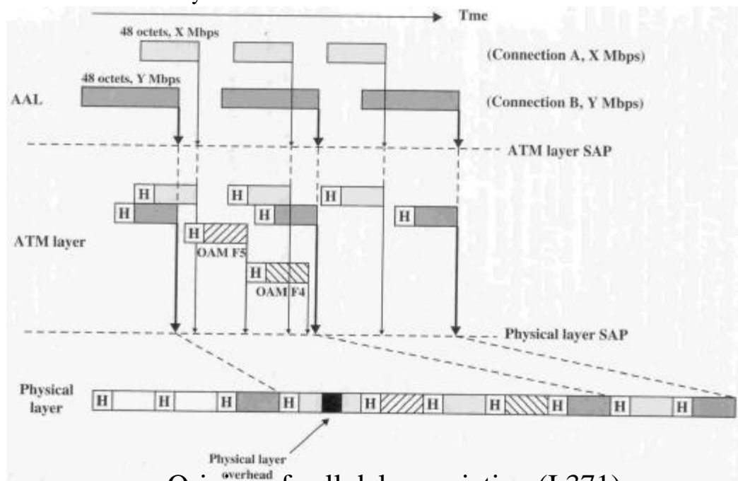
Origins of cell delay variation (I.371)
