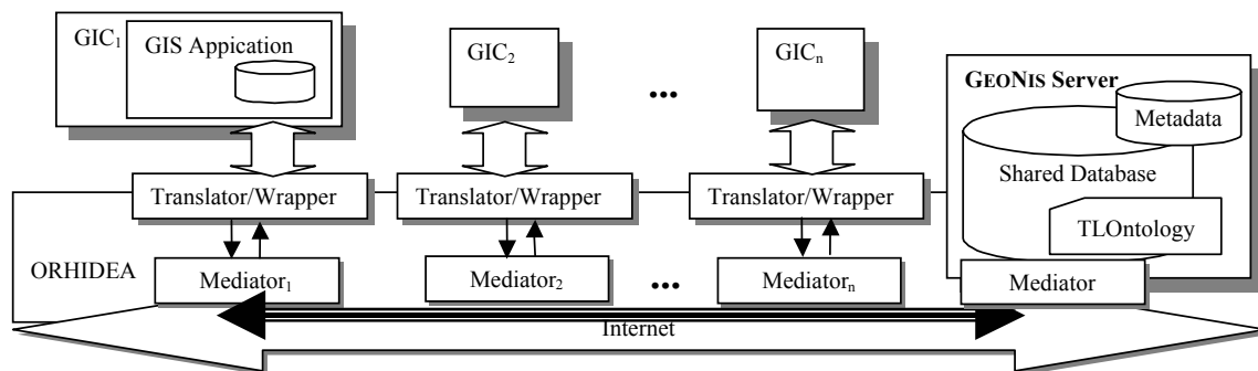
Figure 1. GEONIS interoperability framework architecture
