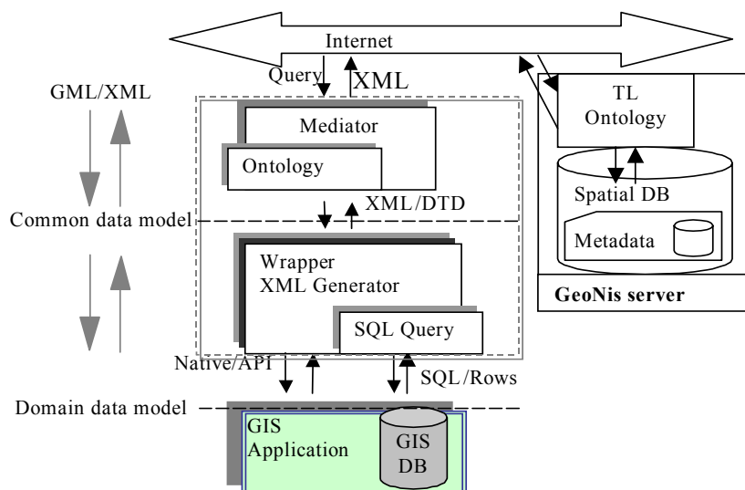
Figure 2. Data flow in GEONIS
