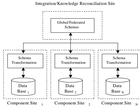
Figure 1. A well-known architecture for global and federated database approach
