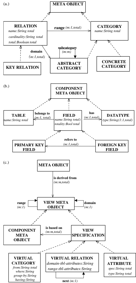
Figure 3. (a.) Meta-schema of Sem-ODM (b.) Meta-schema for a relational database (c.) Mapping from transformed schema (Sem-ODM schema) to component schema (relational schema).
