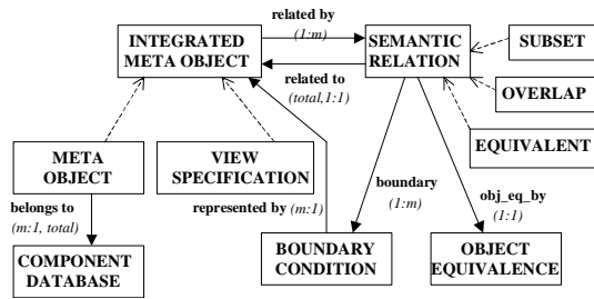
Figure 4. Schema of knowledge base at Integration/Knowledge Reconciliation site
