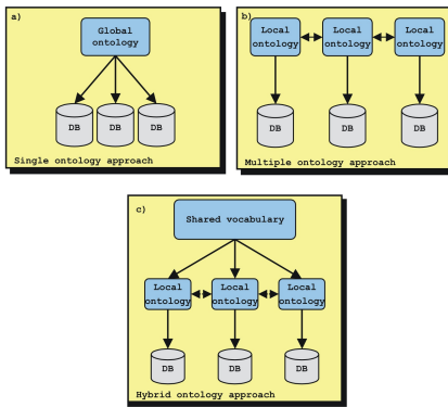
Figure 1: The three possible ways for using ontologies for content explication
