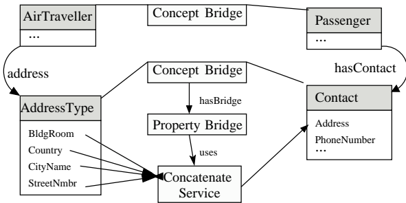
Figure 3: An Example Ontology Mapping through MAFRA
